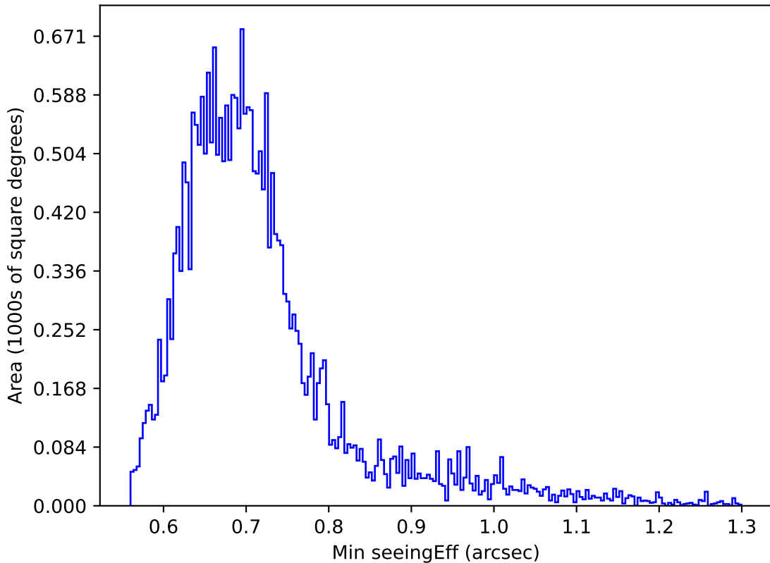
too_ignore_5_4v3.4_10yrs Yr 1 z band: Min seeingEff
