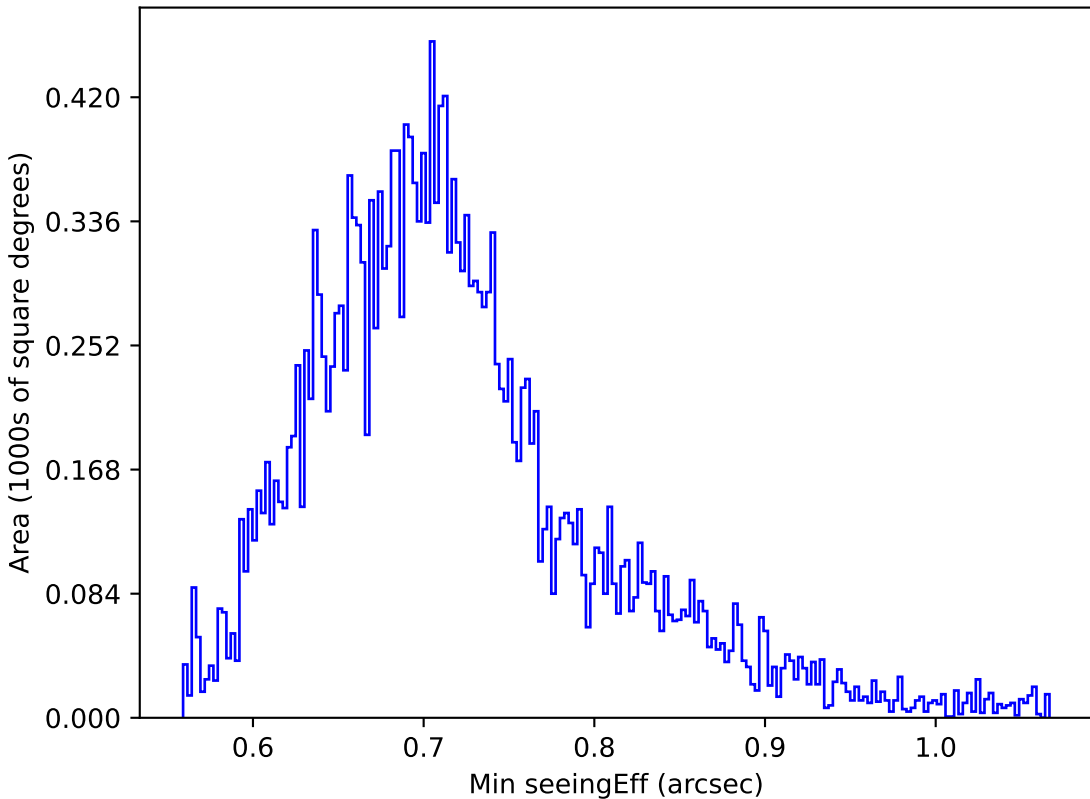
too_ignore_5_4v3.4_10yrs Yr 1 y band: Min seeingEff
