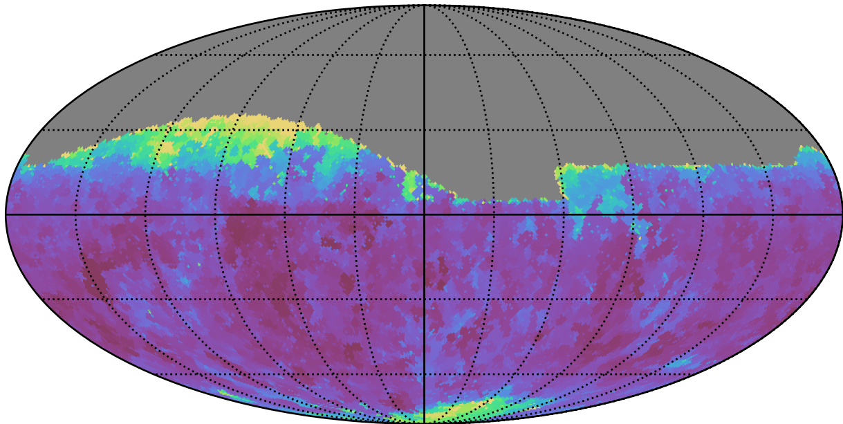
too_ignore_5_4v3.4_10yrs Yr 1 r band: Min seeingEff
