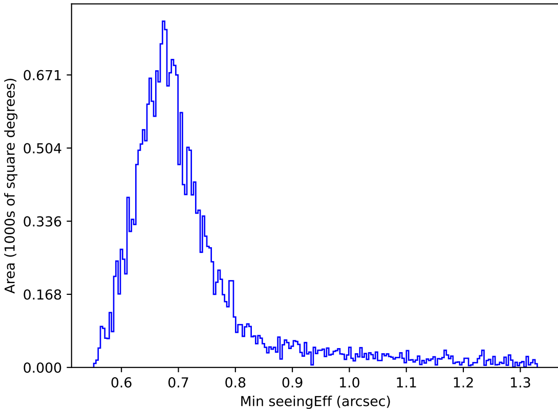
too_ignore_5_4v3.4_10yrs Yr 1 r band: Min seeingEff
