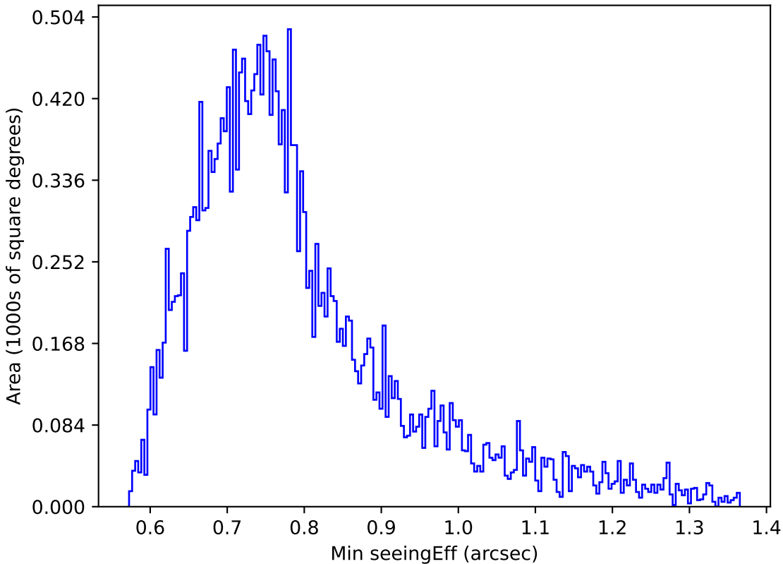
too_ignore_5_4v3.4_10yrs Yr 1 g band: Min seeingEff
