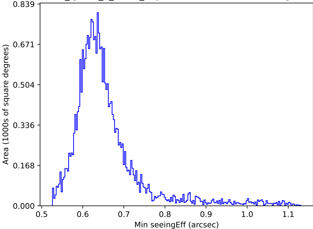
too_ignore_5_4v3.4_10yrs Yr 1 all bands: Min seeingEff
