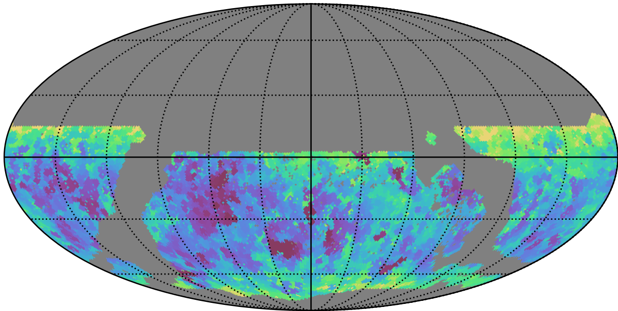
too_ignore_5_4v3.4_10yrs WFD z band: Min seeingEff
