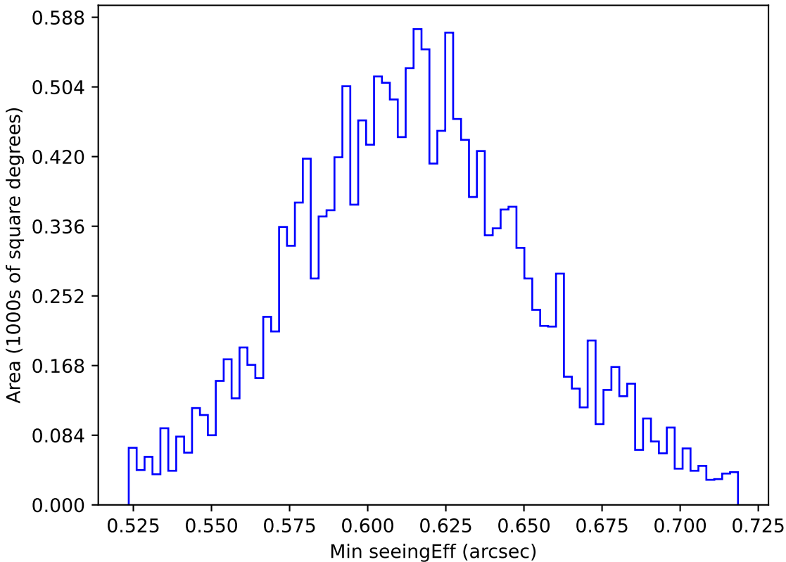
too_ignore_5_4v3.4_10yrs WFD z band: Min seeingEff
