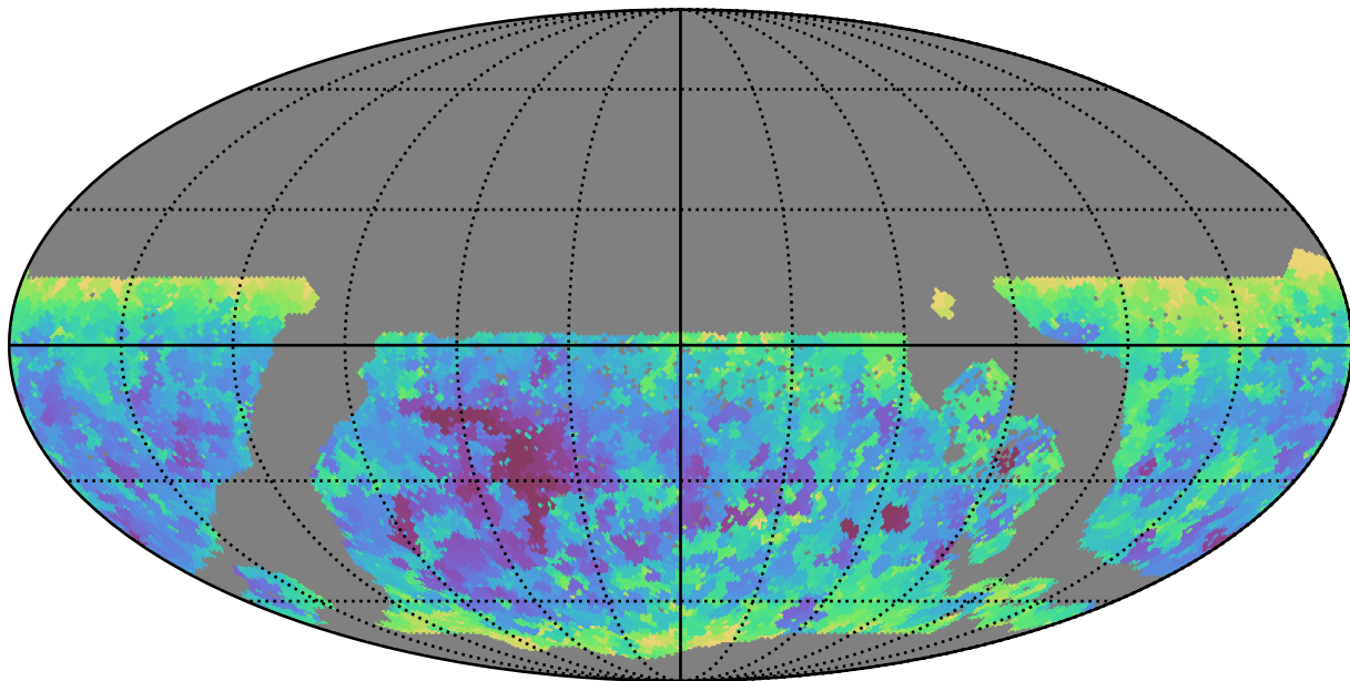
too_ignore_5_4v3.4_10yrs WFD y band: Min seeingEff
