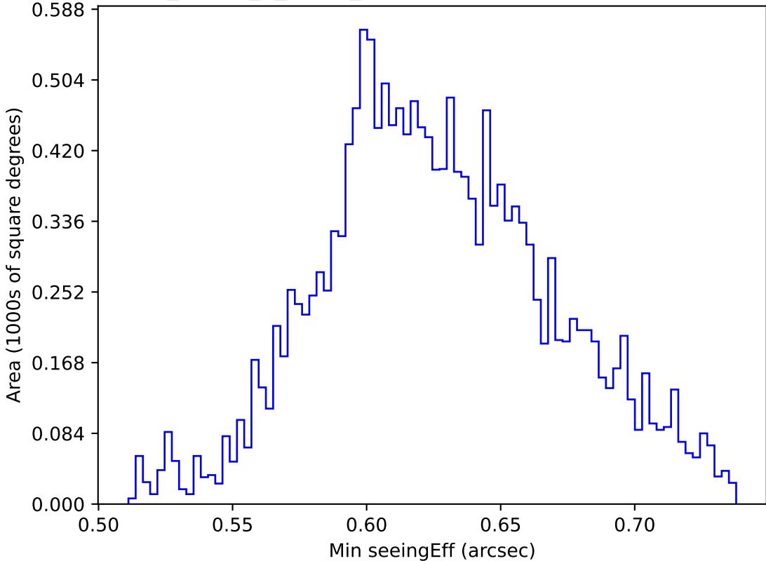
too_ignore_5_4v3.4_10yrs WFD y band: Min seeingEff
