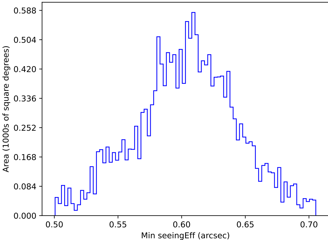
too_ignore_5_4v3.4_10yrs WFD i band: Min seeingEff
