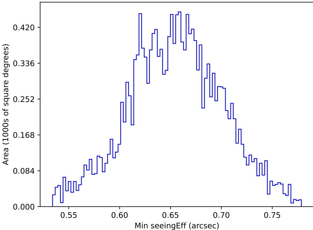
too_ignore_5_4v3.4_10yrs WFD g band: Min seeingEff
