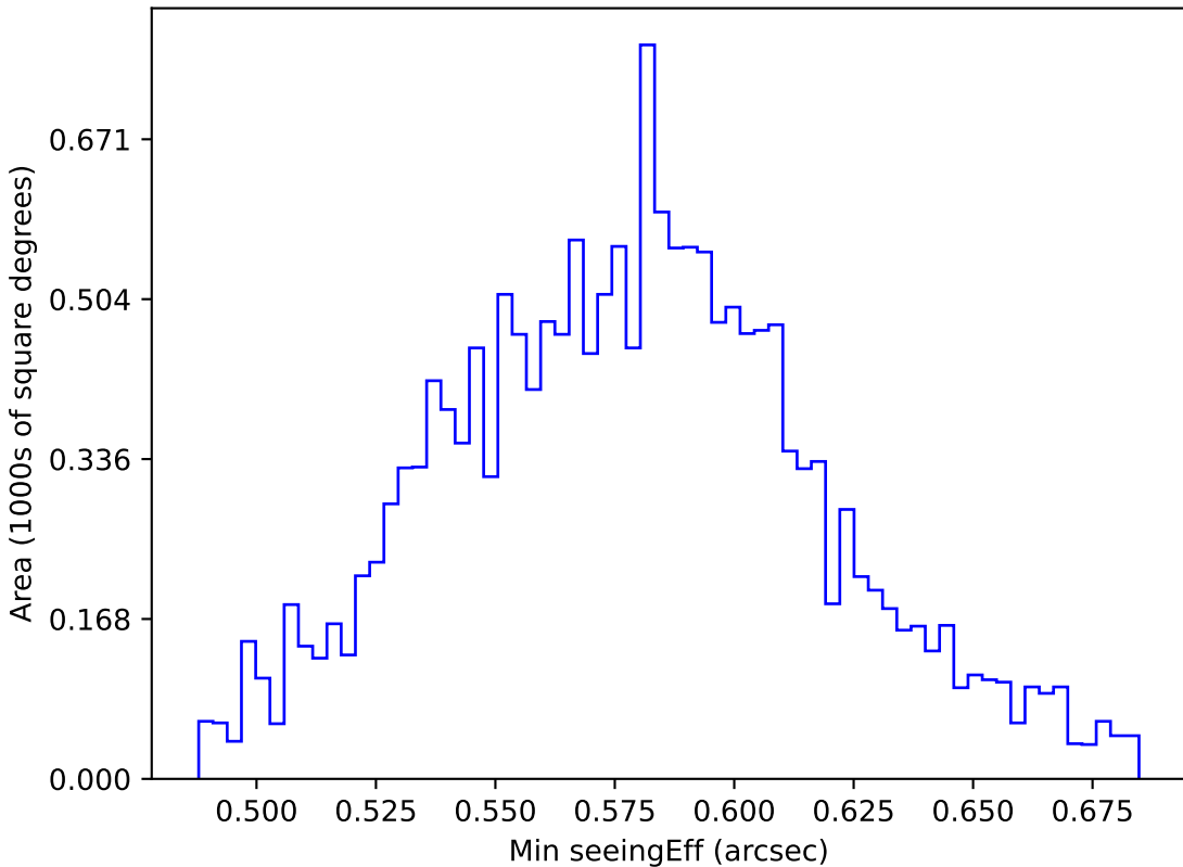
too_ignore_5_4v3.4_10yrs WFD all bands: Min seeingEff
