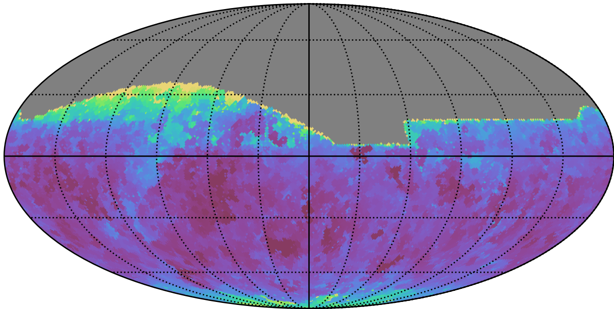
too_ignore_5_4v3.4_10yrs All sky z band: Min seeingEff
