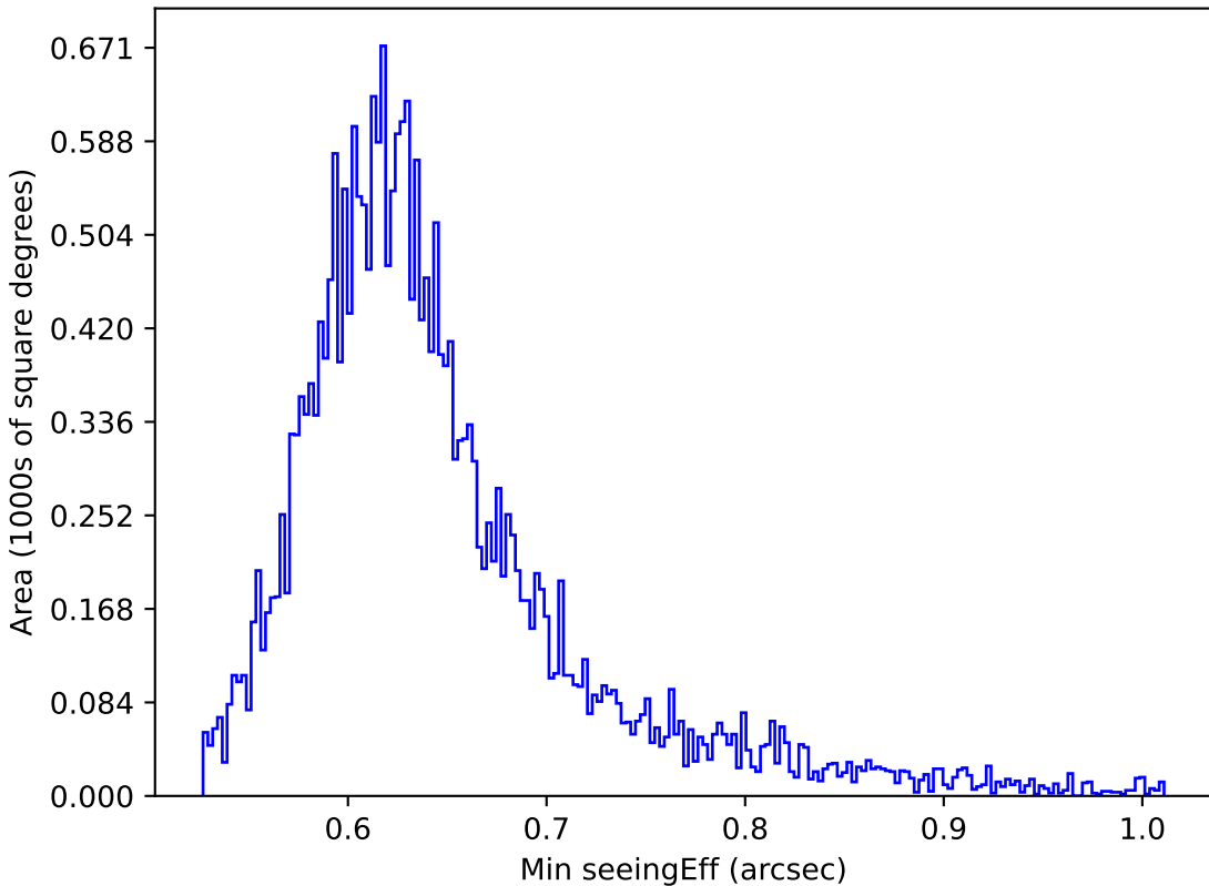
too_ignore_5_4v3.4_10yrs All sky z band: Min seeingEff
