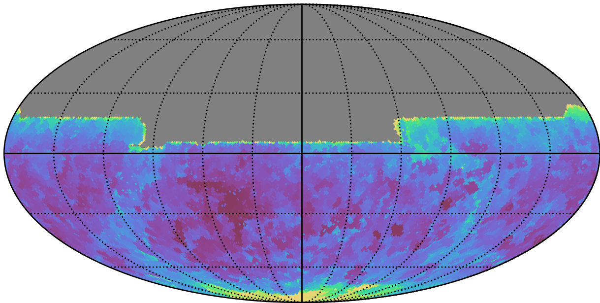
too_ignore_5_4v3.4_10yrs All sky y band: Min seeingEff
