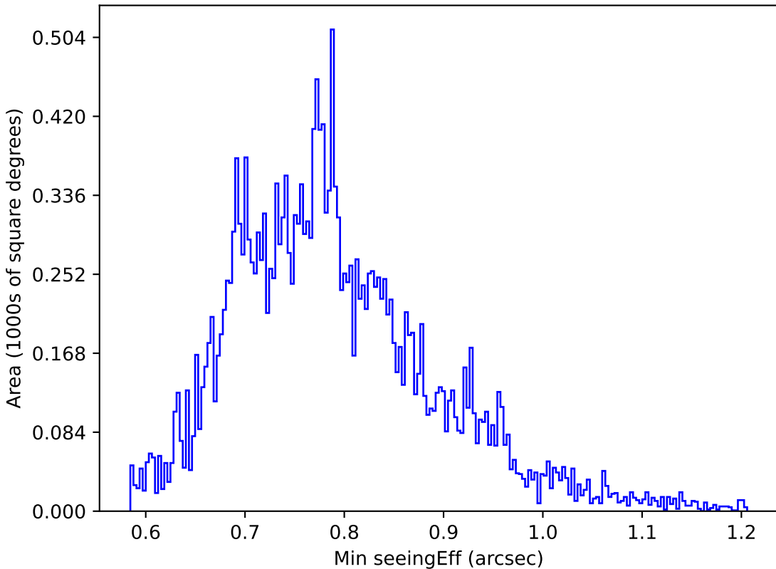
too_ignore_5_4v3.4_10yrs All sky u band: Min seeingEff
