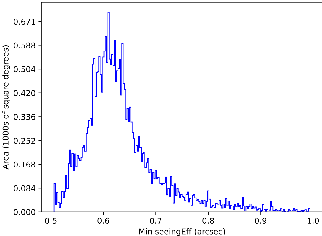
too_ignore_5_4v3.4_10yrs All sky i band: Min seeingEff
