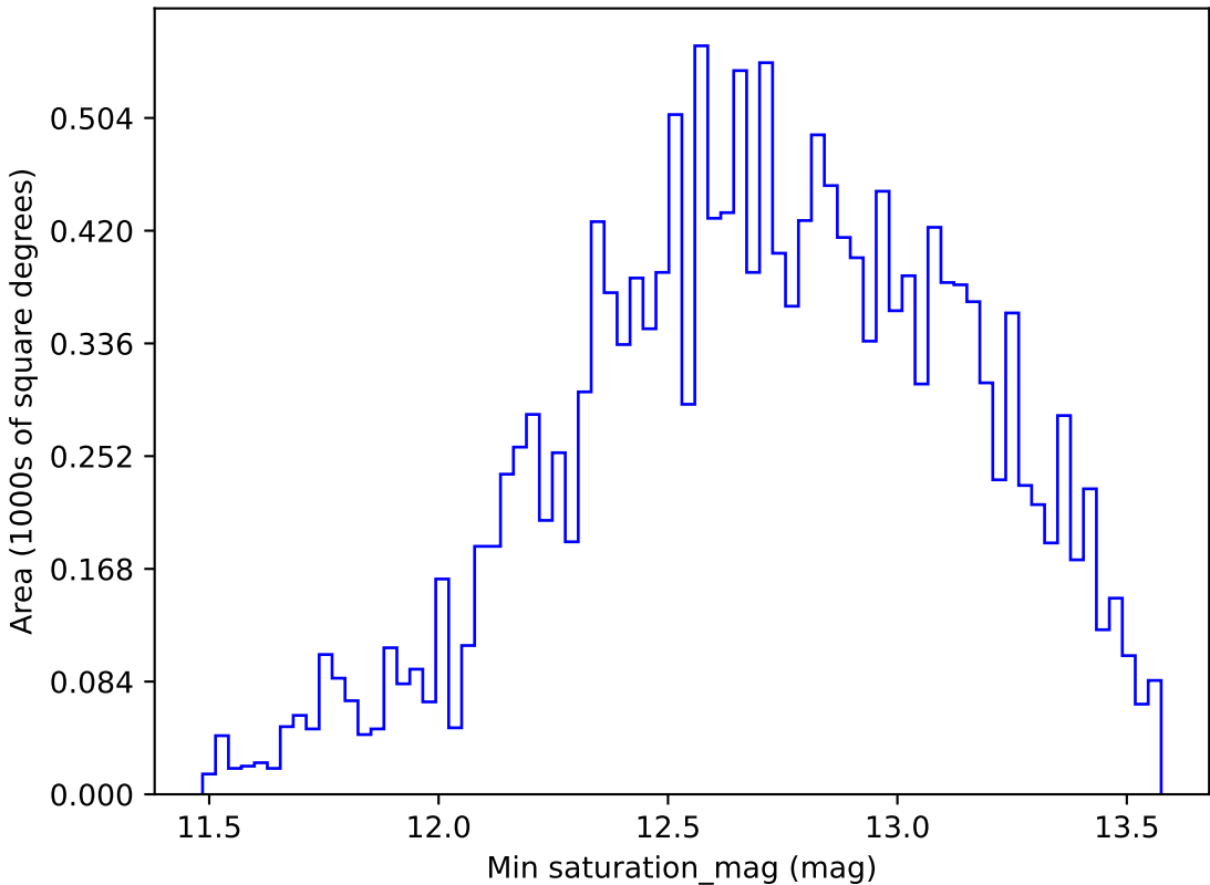
too_ignore_5_4v3.4_10yrs WFD g band: Min saturation_mag
