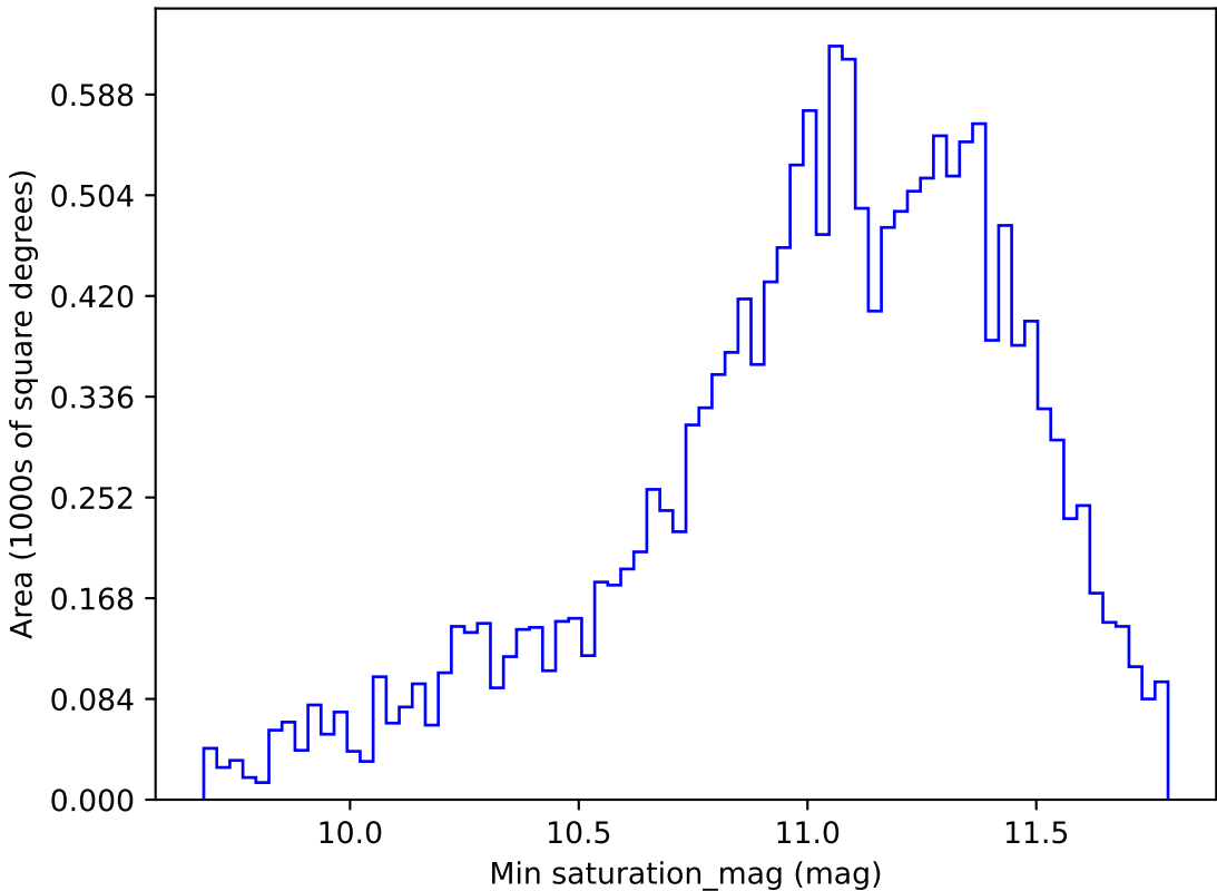
too_ignore_5_4v3.4_10yrs WFD all bands: Min saturation_mag
