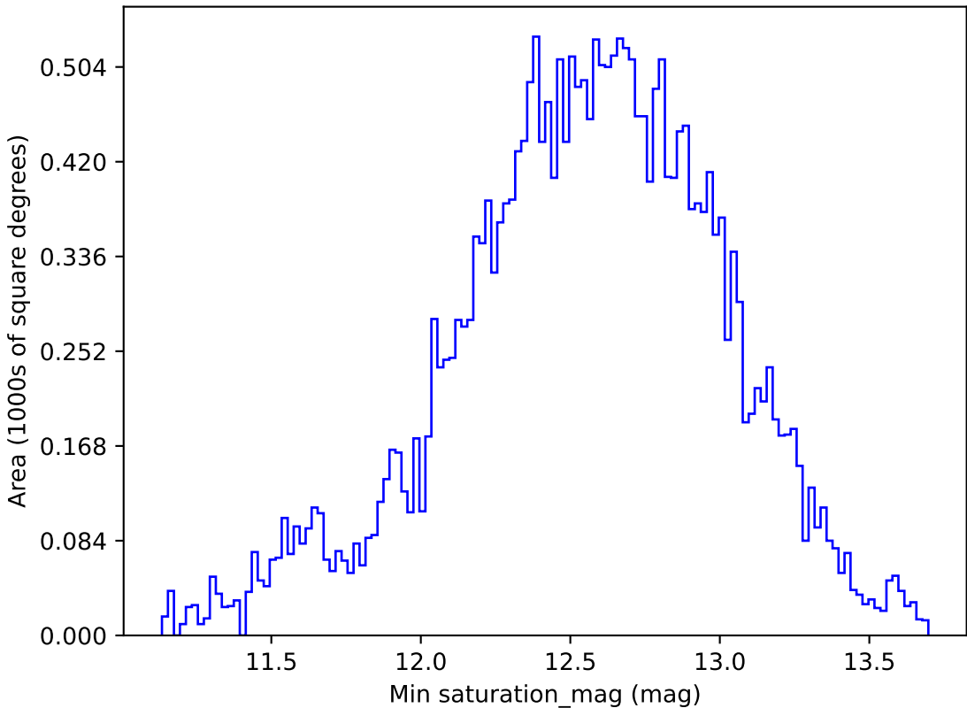
too_ignore_5_4v3.4_10yrs All sky r band: Min saturation_mag
