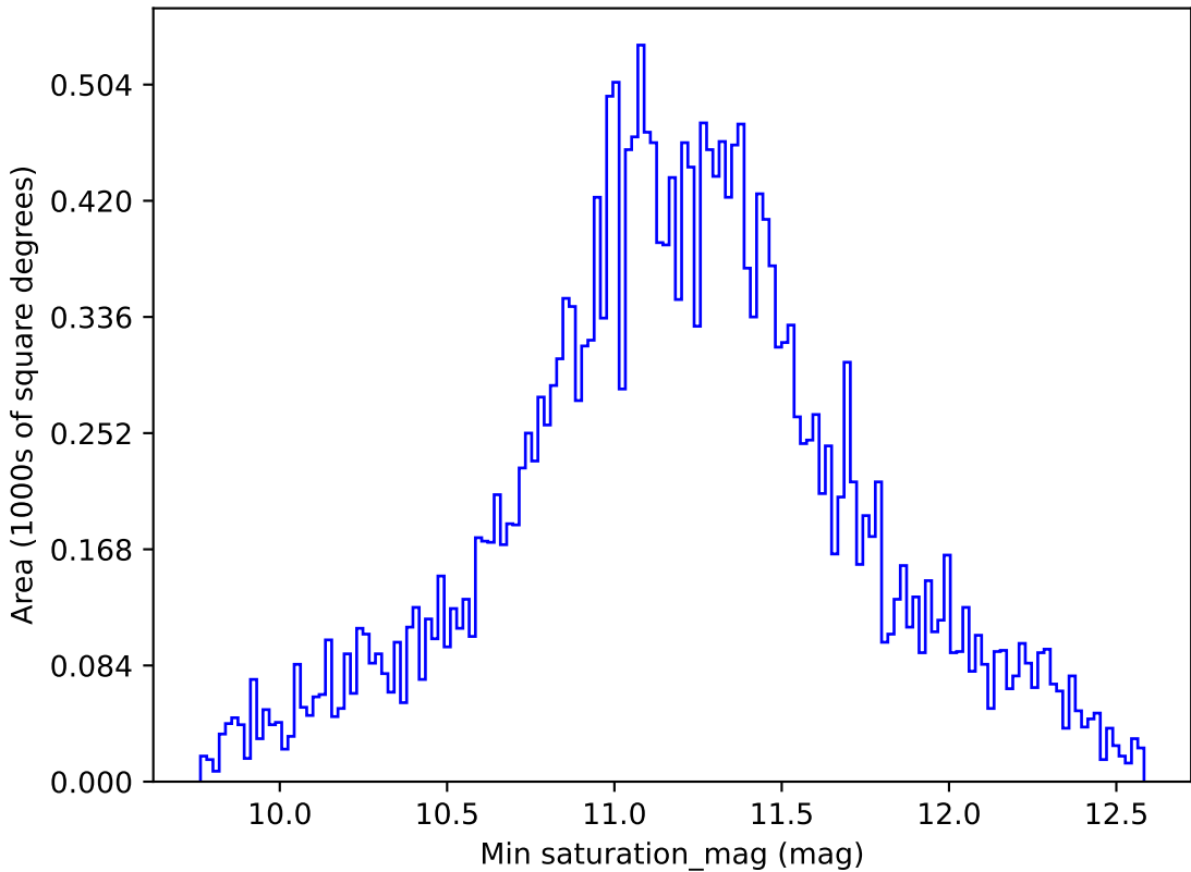
too_ignore_5_4v3.4_10yrs All sky all bands: Min saturation_mag
