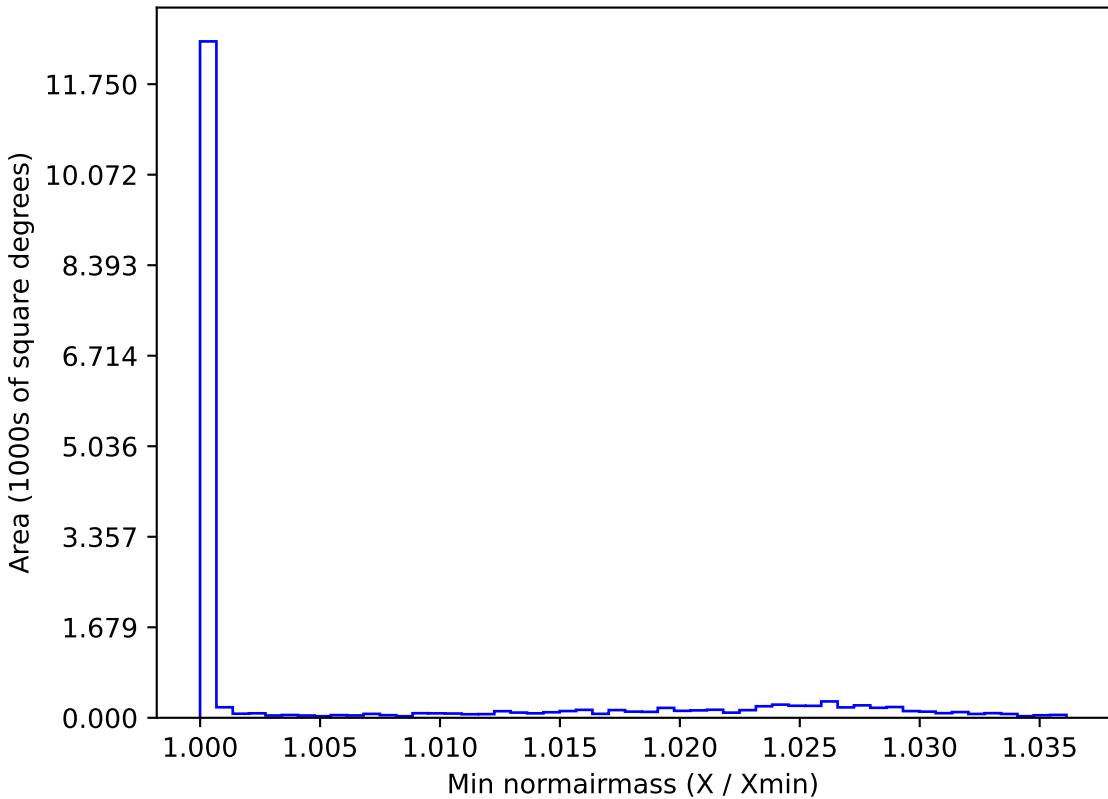
too_ignore_5_4v3.4_10yrs WFD z band: Min normairmass
