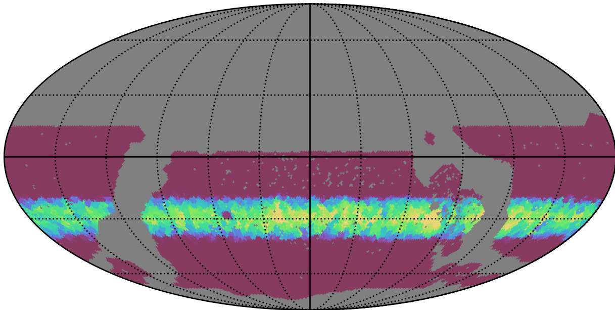
too_ignore_5_4v3.4_10yrs WFD r band: Min normairmass
