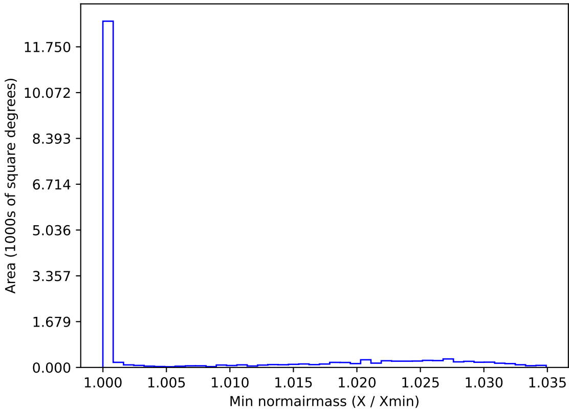
too_ignore_5_4v3.4_10yrs WFD i band: Min normairmass
