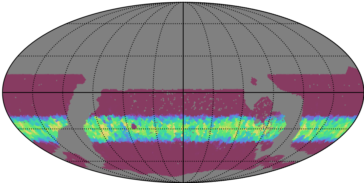
too_ignore_5_4v3.4_10yrs WFD g band: Min normairmass
