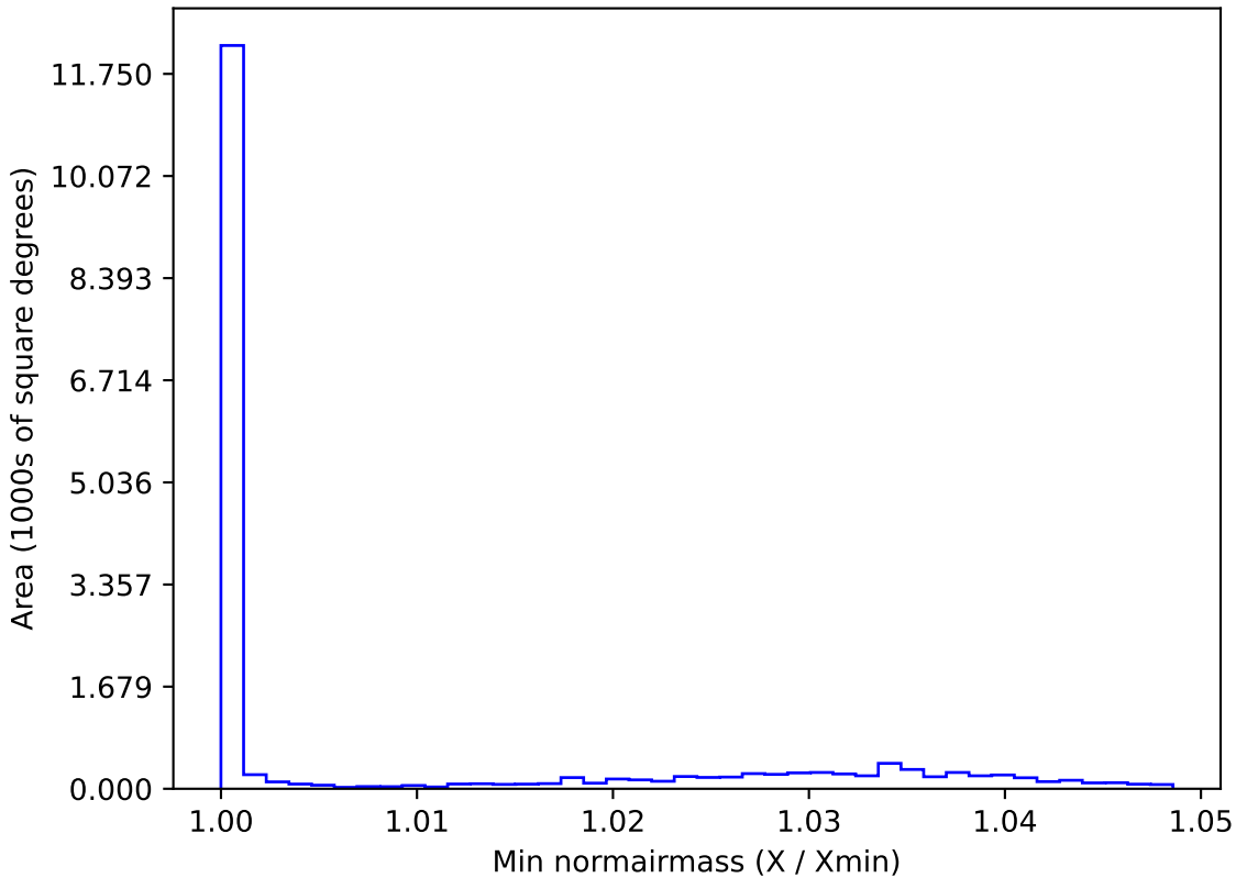
too_ignore_5_4v3.4_10yrs WFD g band: Min normairmass
