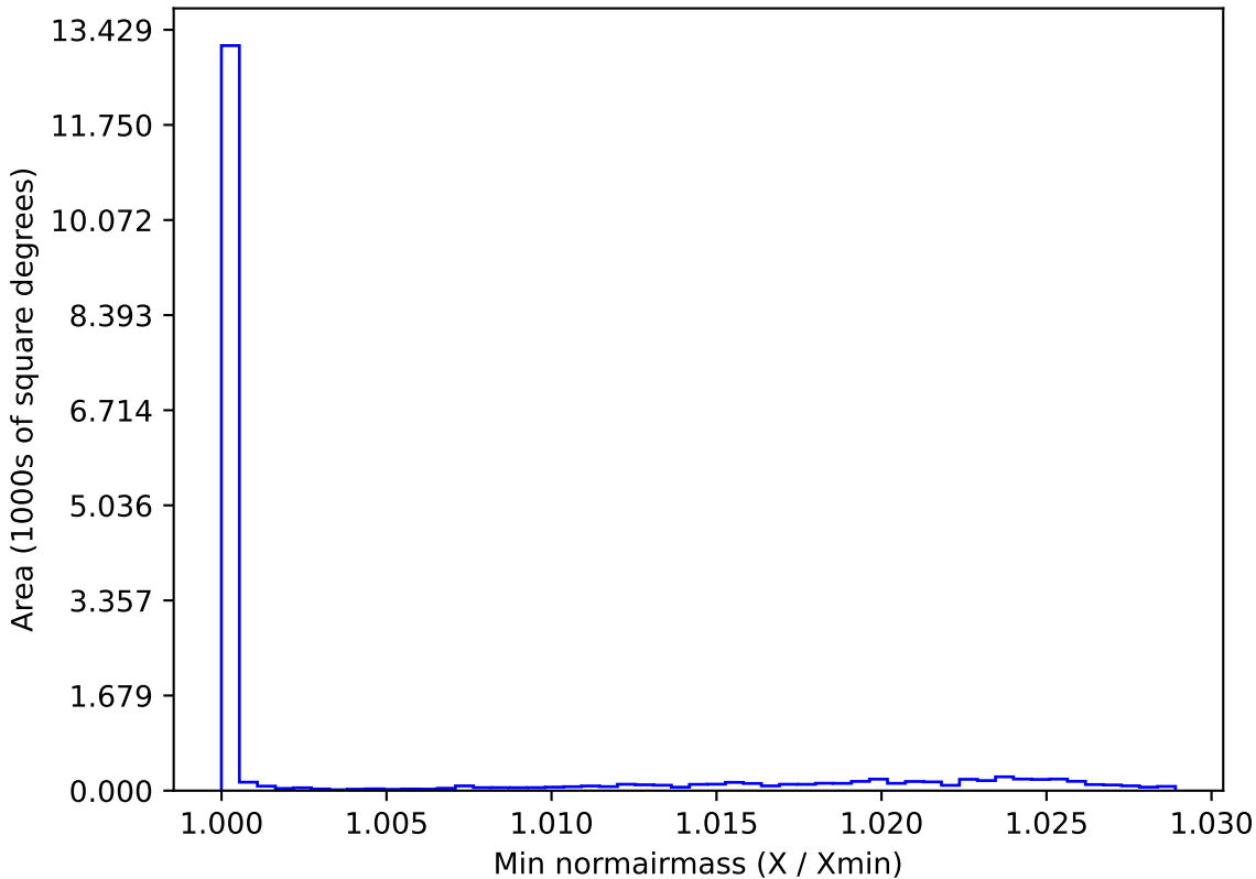
too_ignore_5_4v3.4_10yrs WFD all bands: Min normairmass
