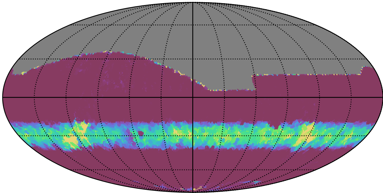
too_ignore_5_4v3.4_10yrs All sky z band: Min normairmass
