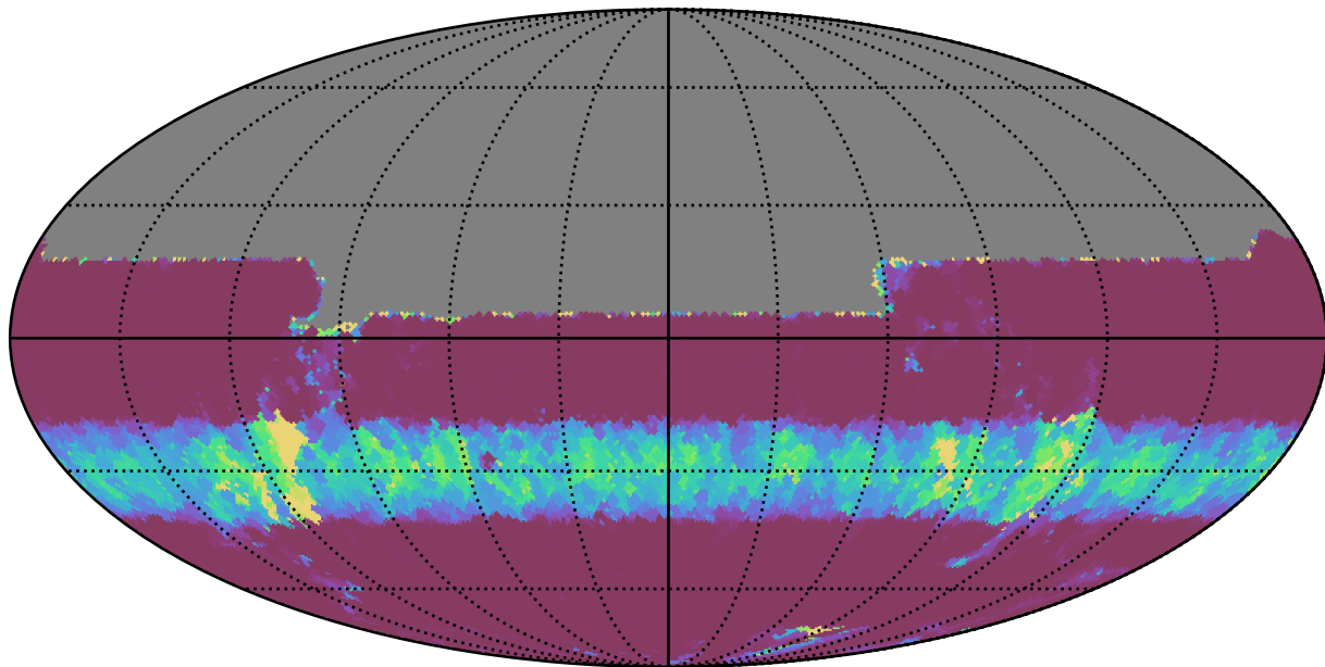
too_ignore_5_4v3.4_10yrs All sky u band: Min normairmass
