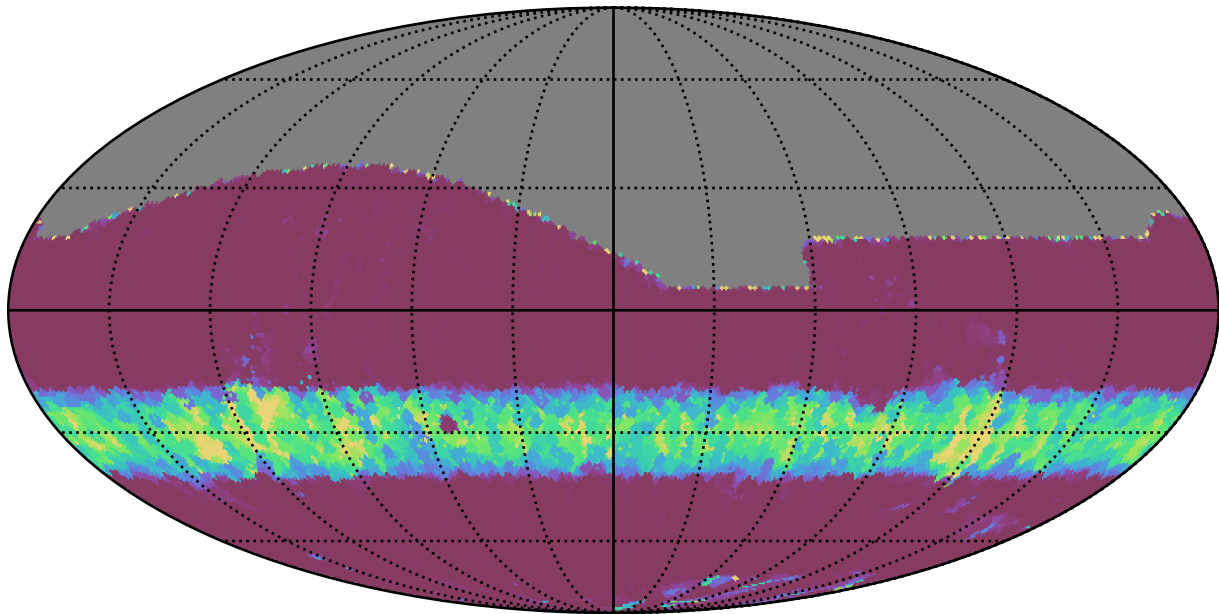
too_ignore_5_4v3.4_10yrs All sky g band: Min normairmass
