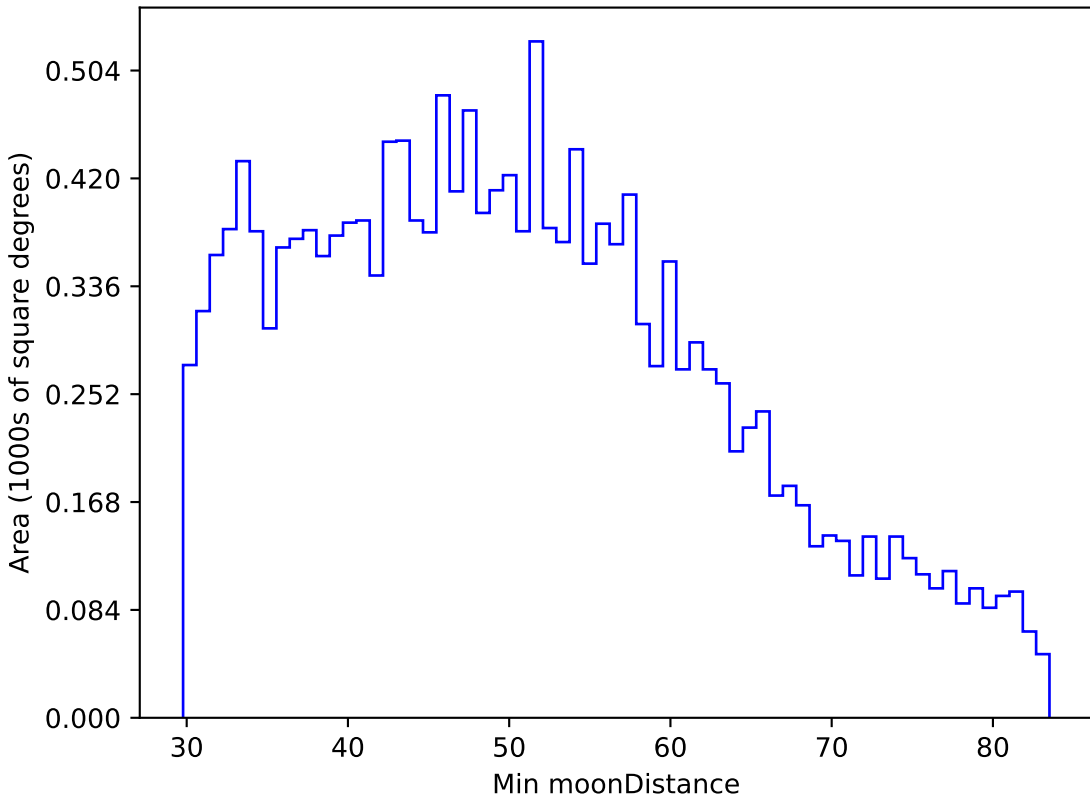
too_ignore_5_4v3.4_10yrs WFD u band: Min moonDistance
