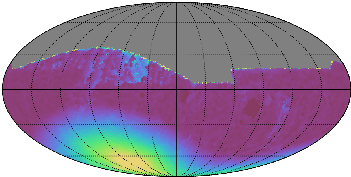
too_ignore_5_4v3.4_10yrs All sky z band: Min moonDistance
