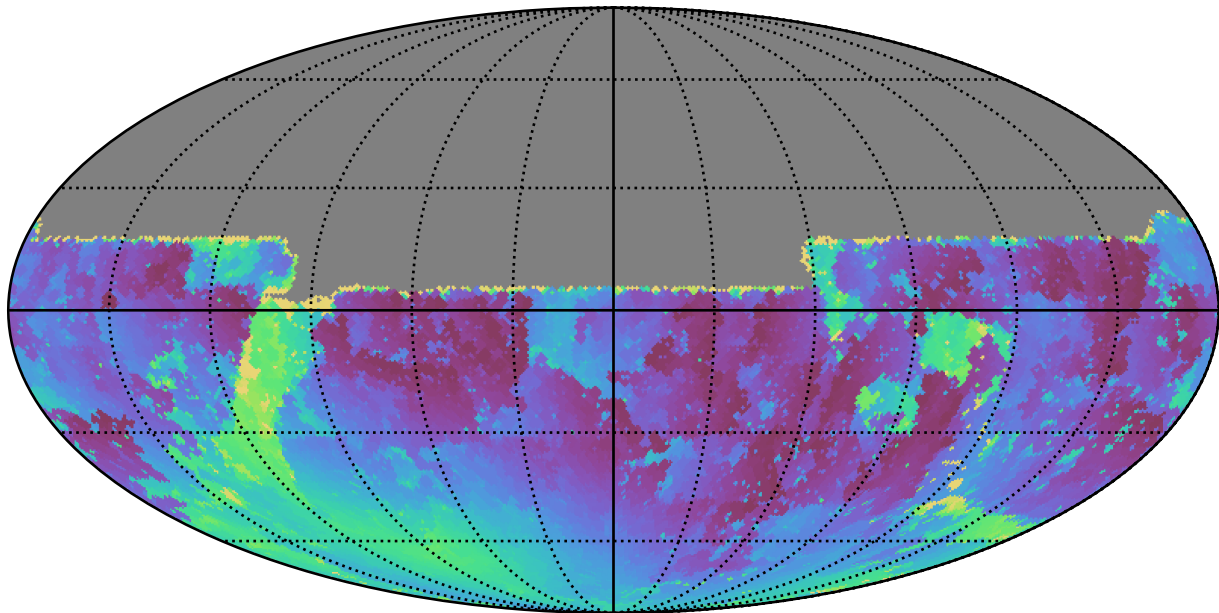
too_ignore_5_4v3.4_10yrs All sky u band: Min moonDistance
