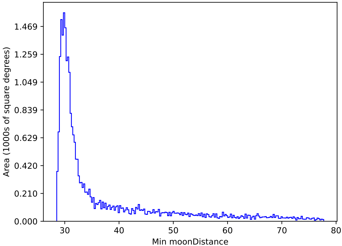
too_ignore_5_4v3.4_10yrs All sky i band: Min moonDistance
