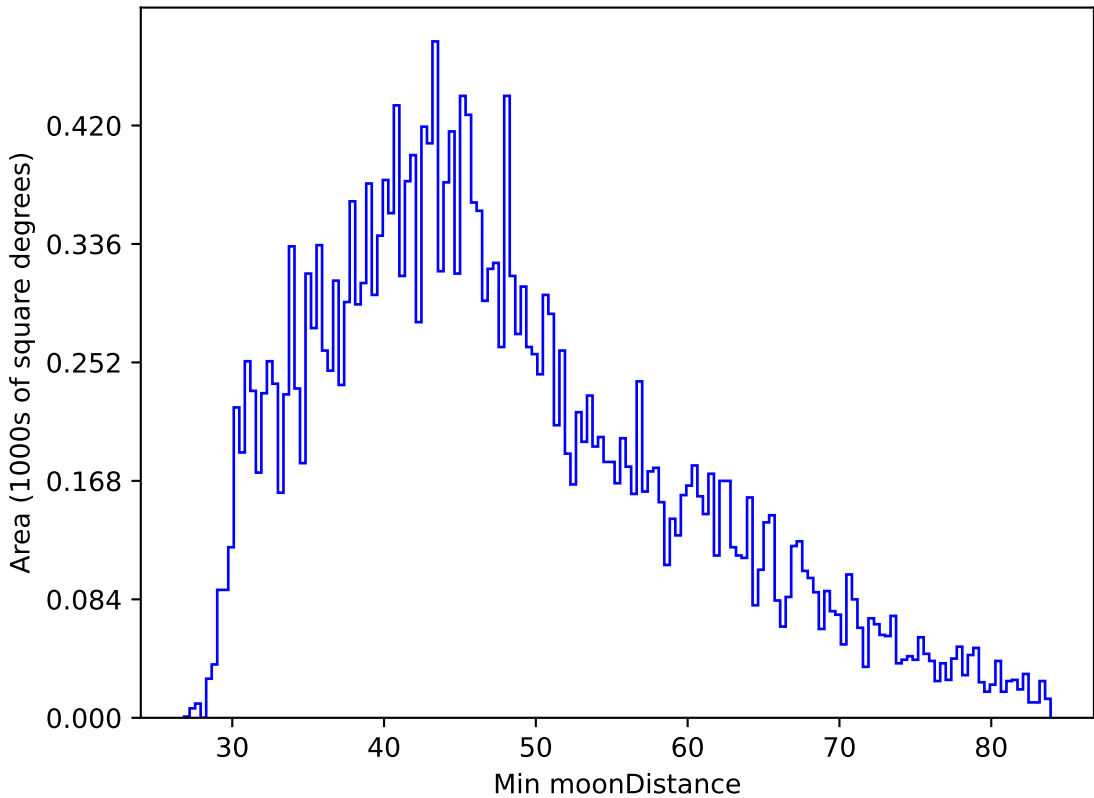
too_ignore_5_4v3.4_10yrs All sky g band: Min moonDistance
