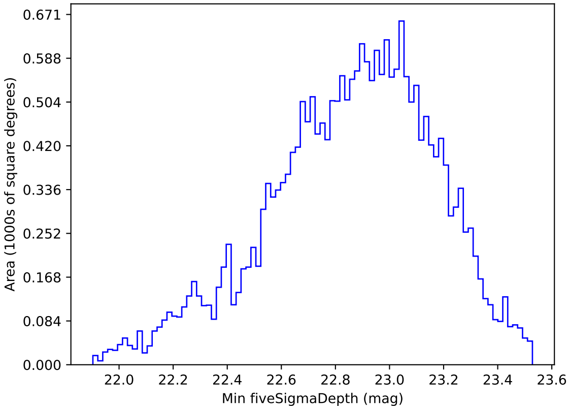
too_ignore_5_4v3.4_10yrs Yr 1 u band: Min fiveSigmaDepth
