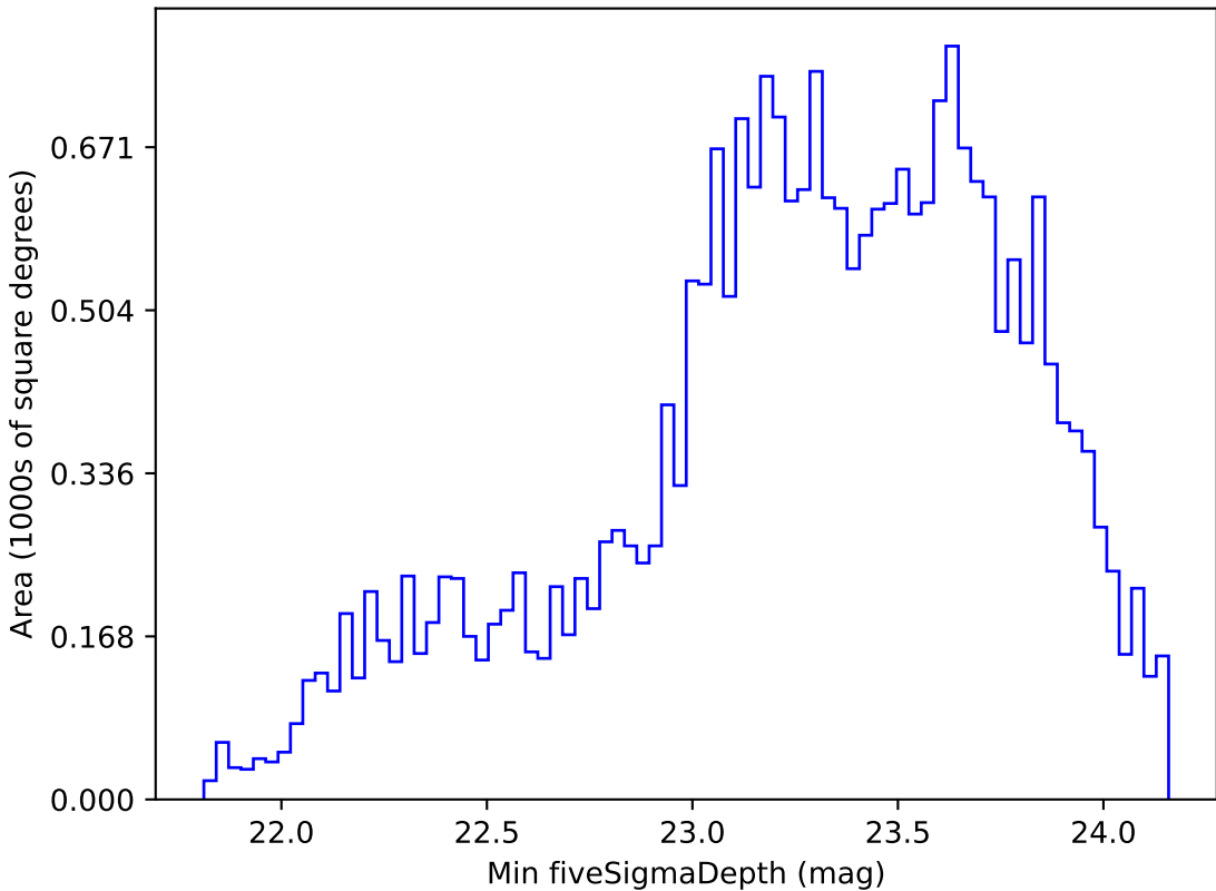
too_ignore_5_4v3.4_10yrs Yr 1 r band: Min fiveSigmaDepth
