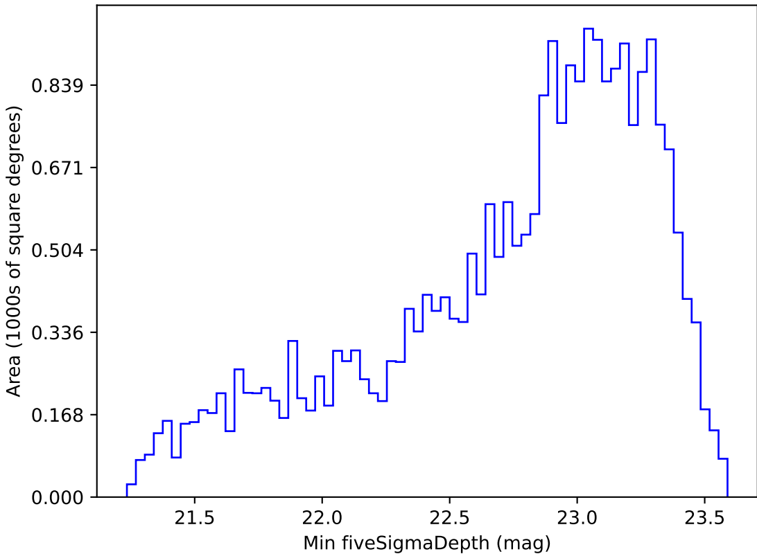
too_ignore_5_4v3.4_10yrs Yr 1 i band: Min fiveSigmaDepth
