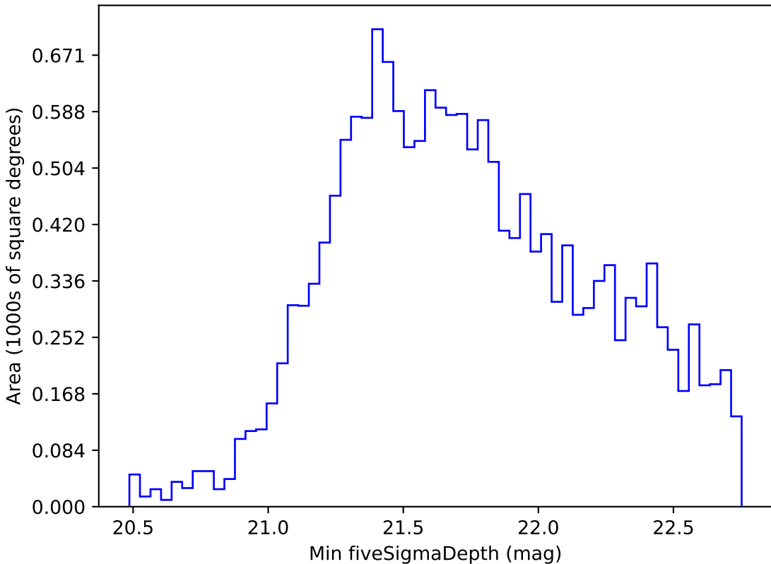
too_ignore_5_4v3.4_10yrs WFD i band: Min fiveSigmaDepth
