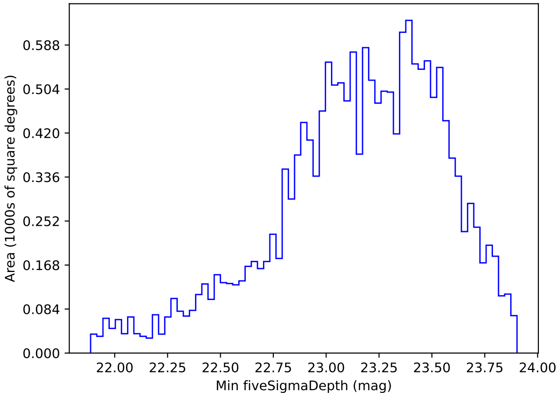
too_ignore_5_4v3.4_10yrs WFD g band: Min fiveSigmaDepth
