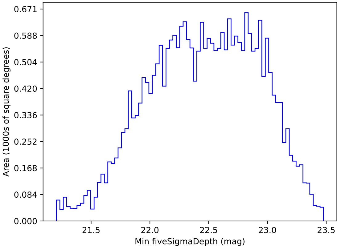
too_ignore_5_4v3.4_10yrs All sky r band: Min fiveSigmaDepth
