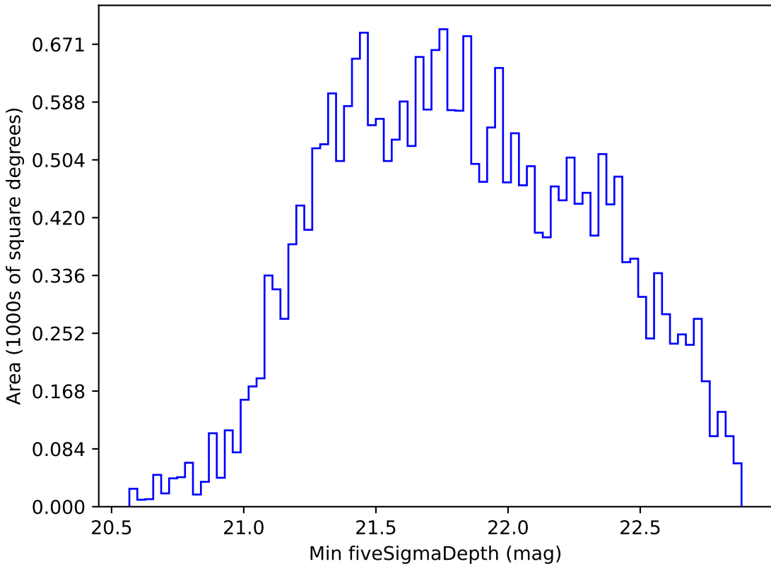
too_ignore_5_4v3.4_10yrs All sky i band: Min fiveSigmaDepth
