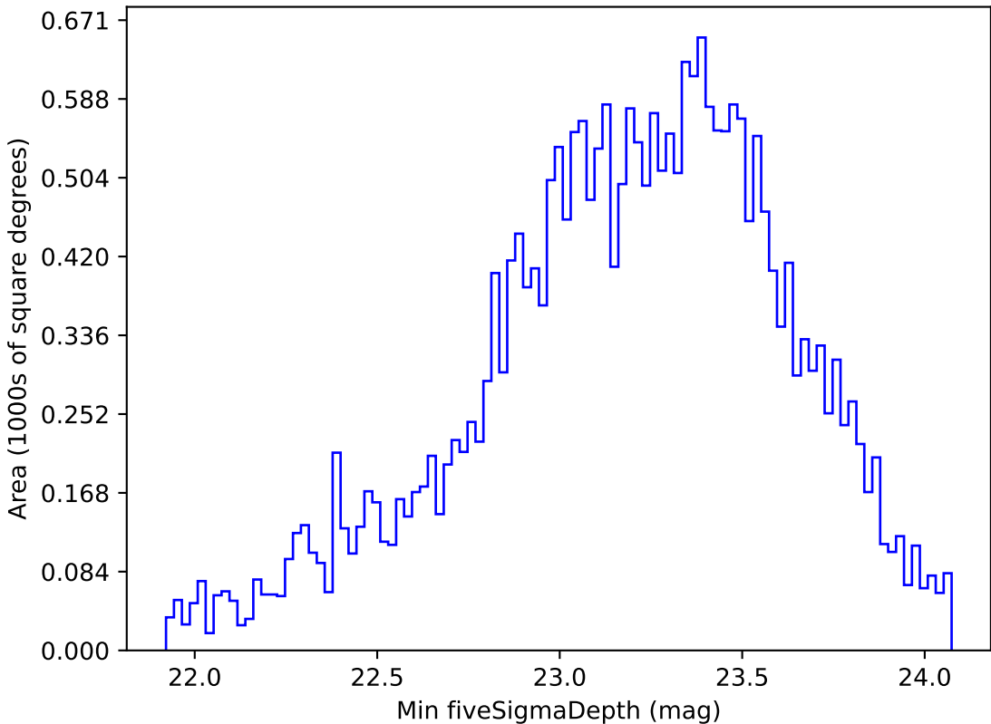
too_ignore_5_4v3.4_10yrs All sky g band: Min fiveSigmaDepth
