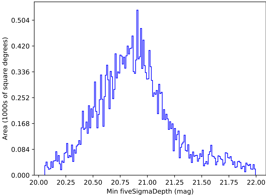
too_ignore_5_4v3.4_10yrs All sky all bands: Min fiveSigmaDepth
