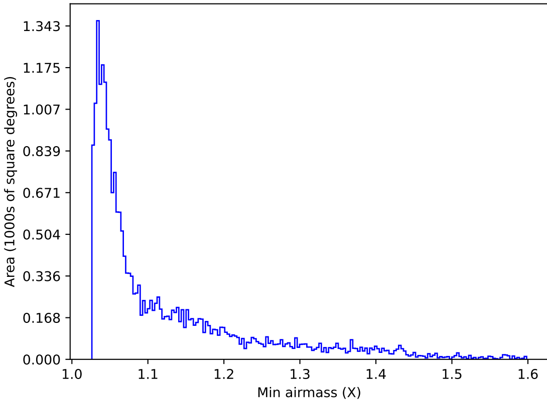
too_ignore_5_4v3.4_10yrs Yr 1 y band: Min airmass
