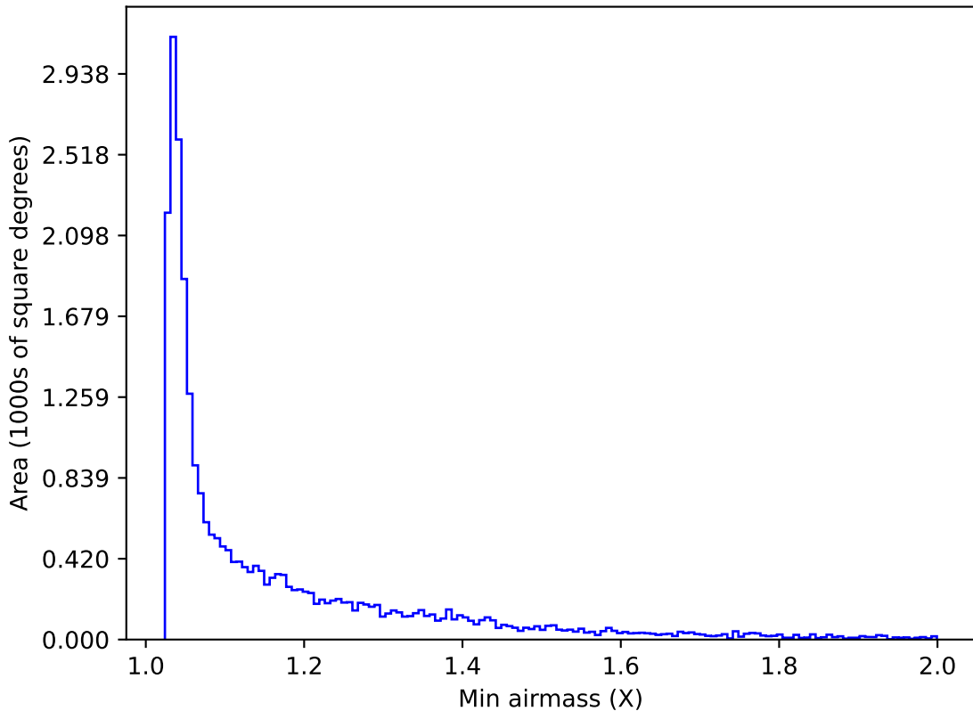
too_ignore_5_4v3.4_10yrs Yr 1 r band: Min airmass
