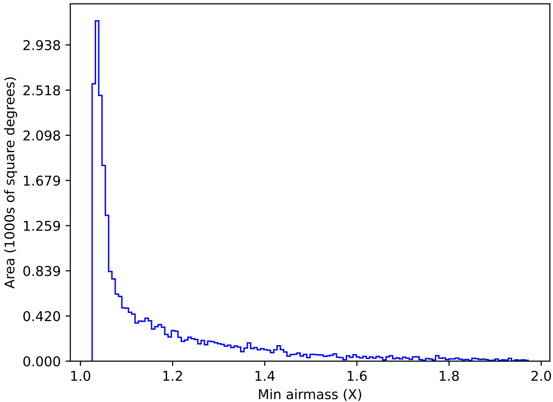
too_ignore_5_4v3.4_10yrs Yr 1 i band: Min airmass
