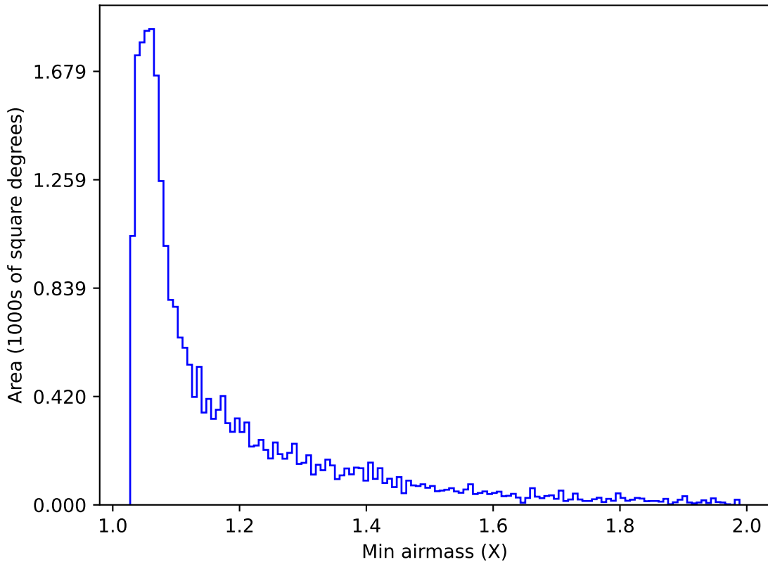
too_ignore_5_4v3.4_10yrs Yr 1 g band: Min airmass
