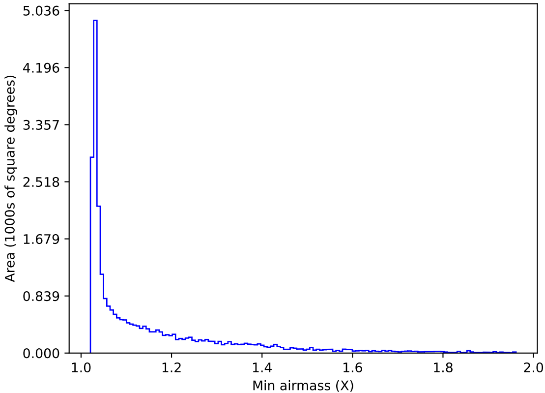
too_ignore_5_4v3.4_10yrs Yr 1 all bands: Min airmass
